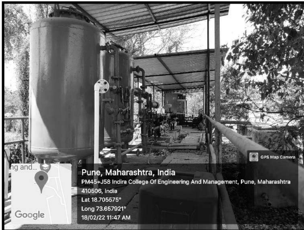
Photo 04: Pressure Sand Filter and other units of Waste Water Treatment Plant
